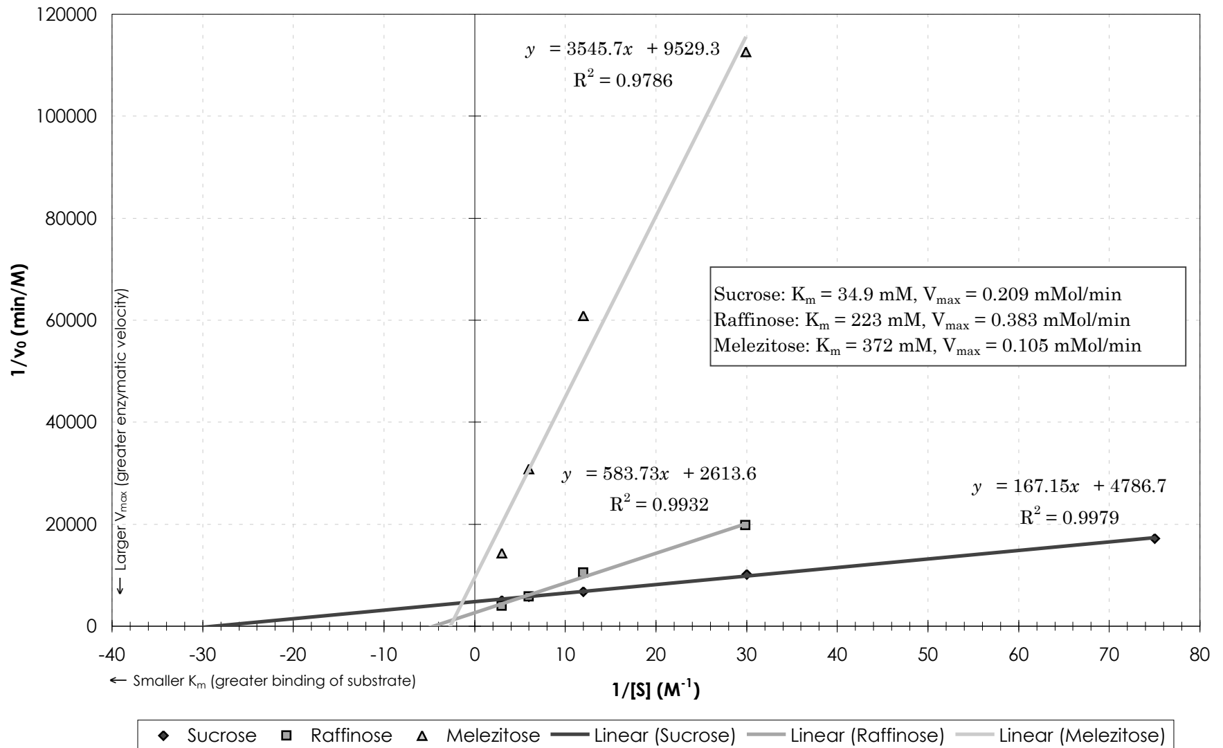
Figure 2. Enzymatic Activity of Invertase with \beta -Fructofuranosides at 20 °C and pH 4.5
