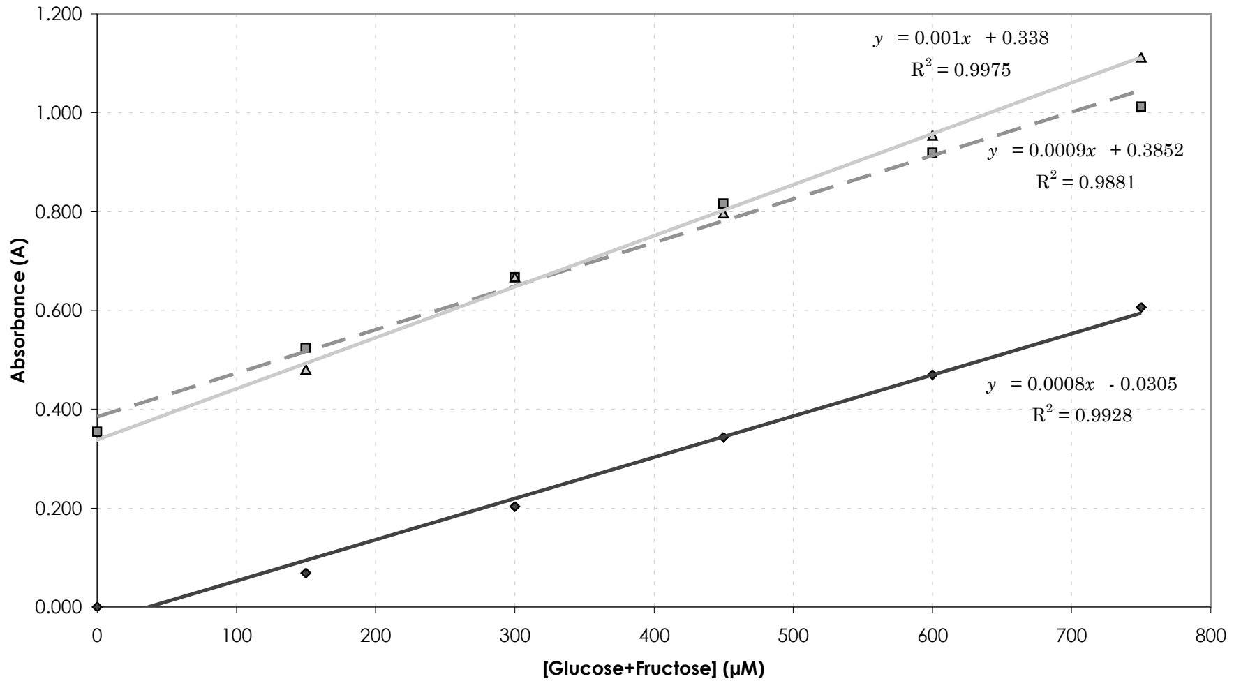
Figure 1. Standard Curves for Determination of Total Reducing Sugars
